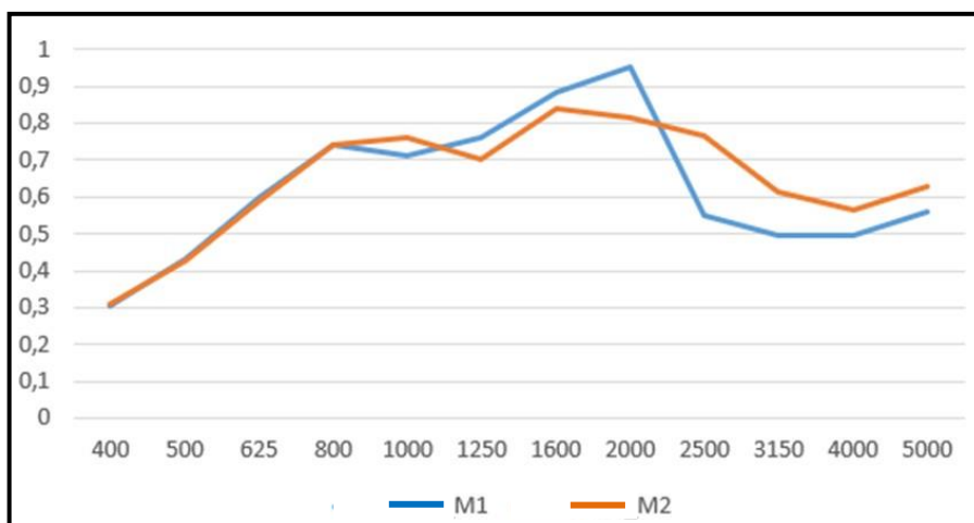
Luftschallabsorption
